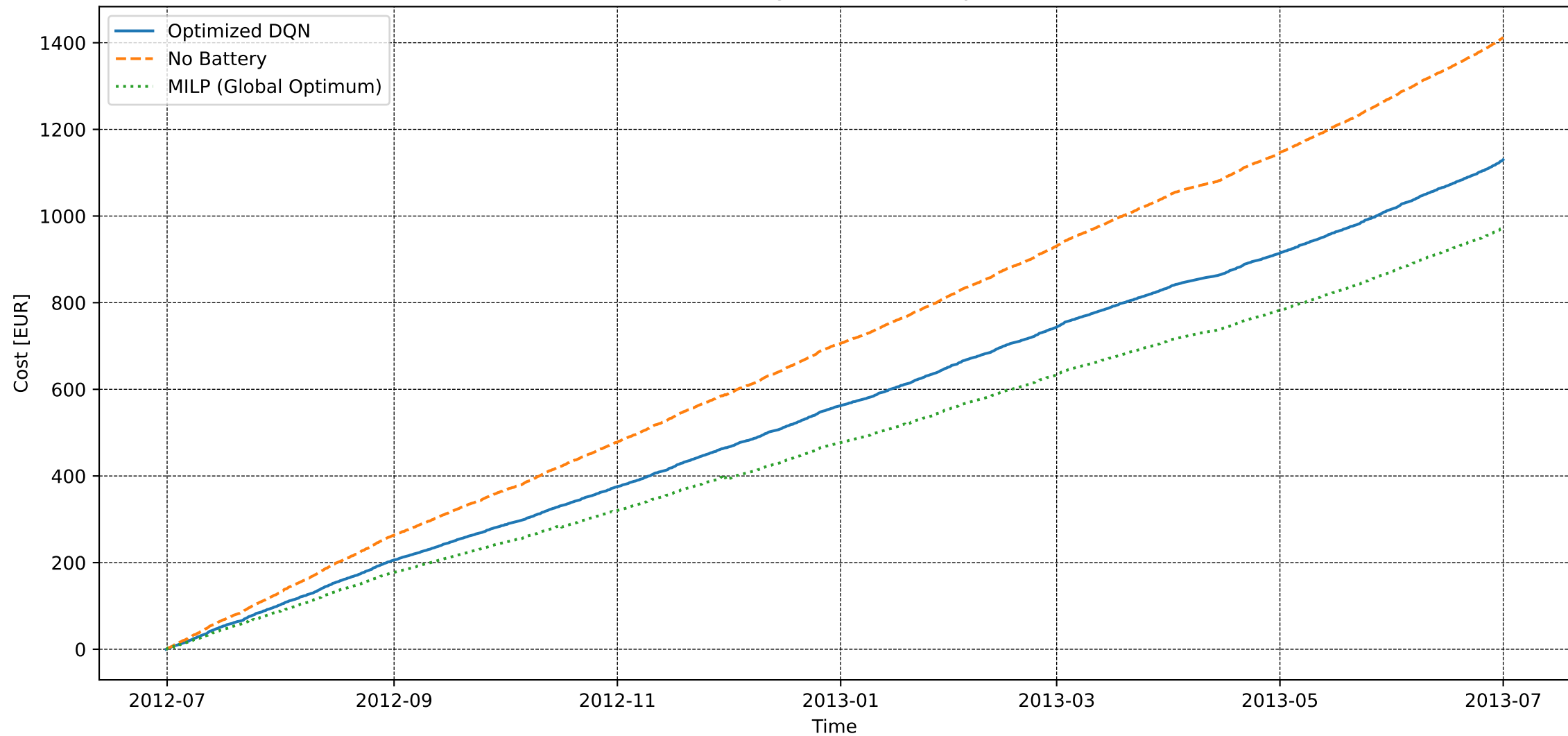
User 67 - Extended Convergence - Electricity Cost [DQN vs MILP]
